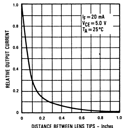
Coupling Characteristics of OP145 and OP555
